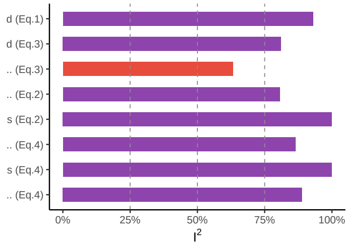
Main models
